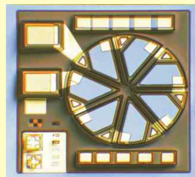
Top view of the planar photovoltaic array
