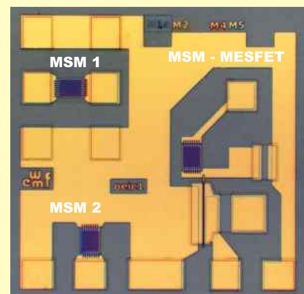
MSM-MESFET Photoreceiver
